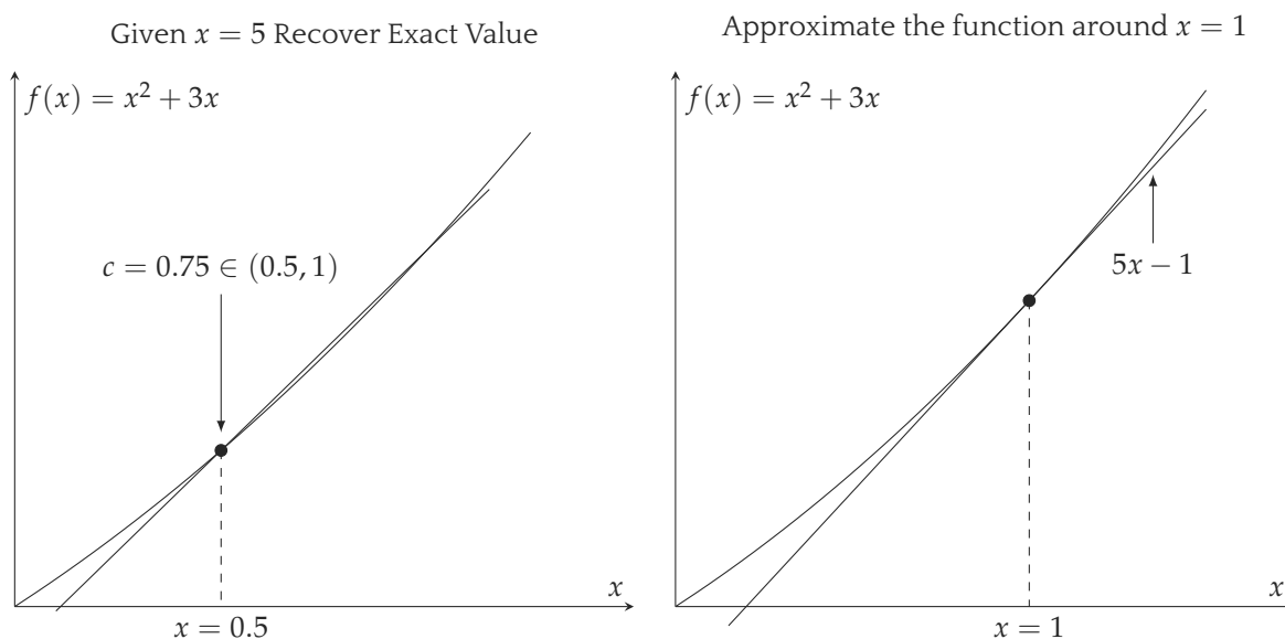
Figure 2: Visualizing Taylor's Theorem
